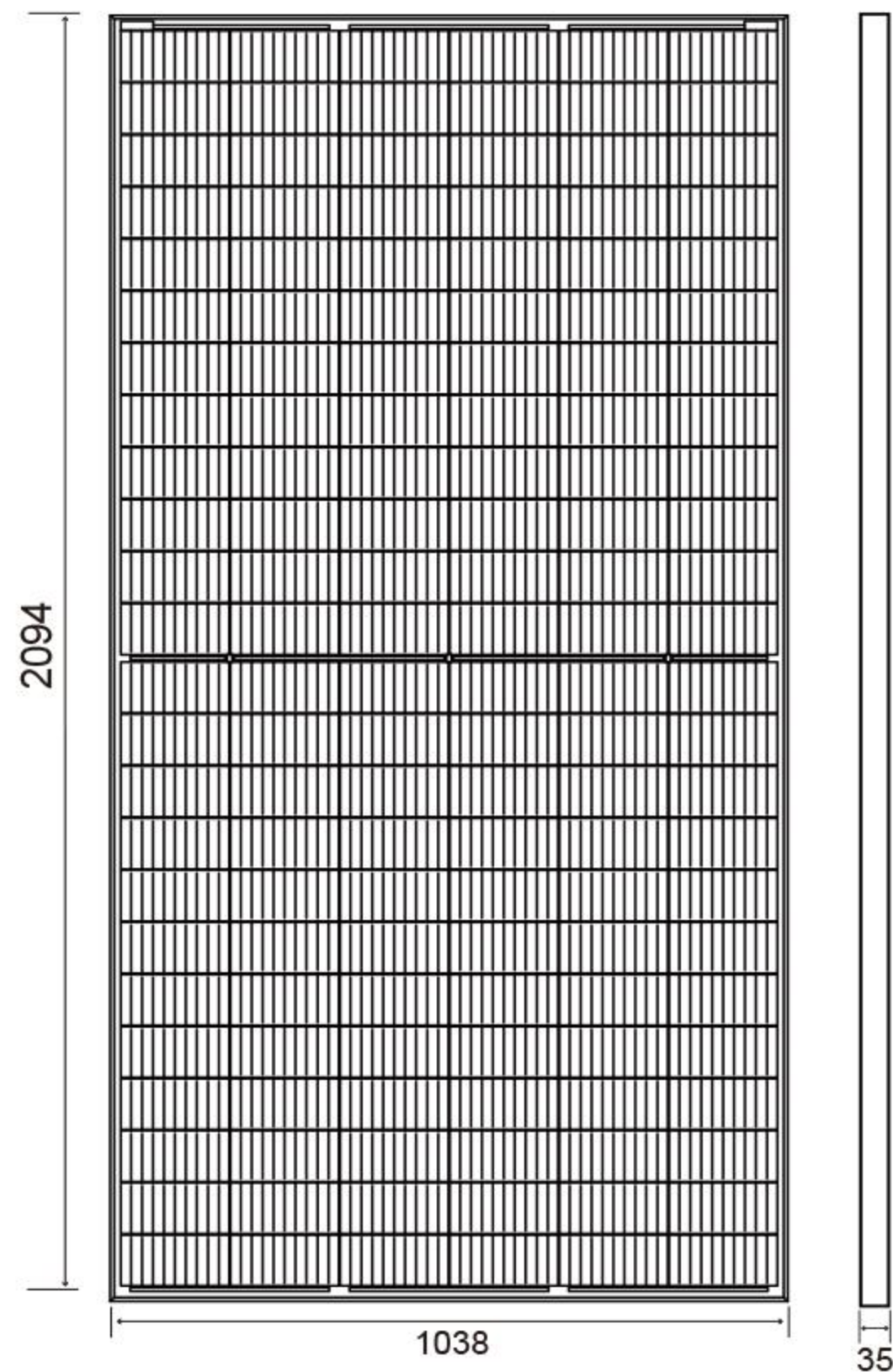
Dimension of PV Modules Unit: mm
