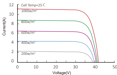
Current-Voltage Curve (RS7K-370M)
