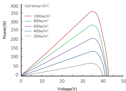
Power-Voltage Curve (RS7K-370M)
