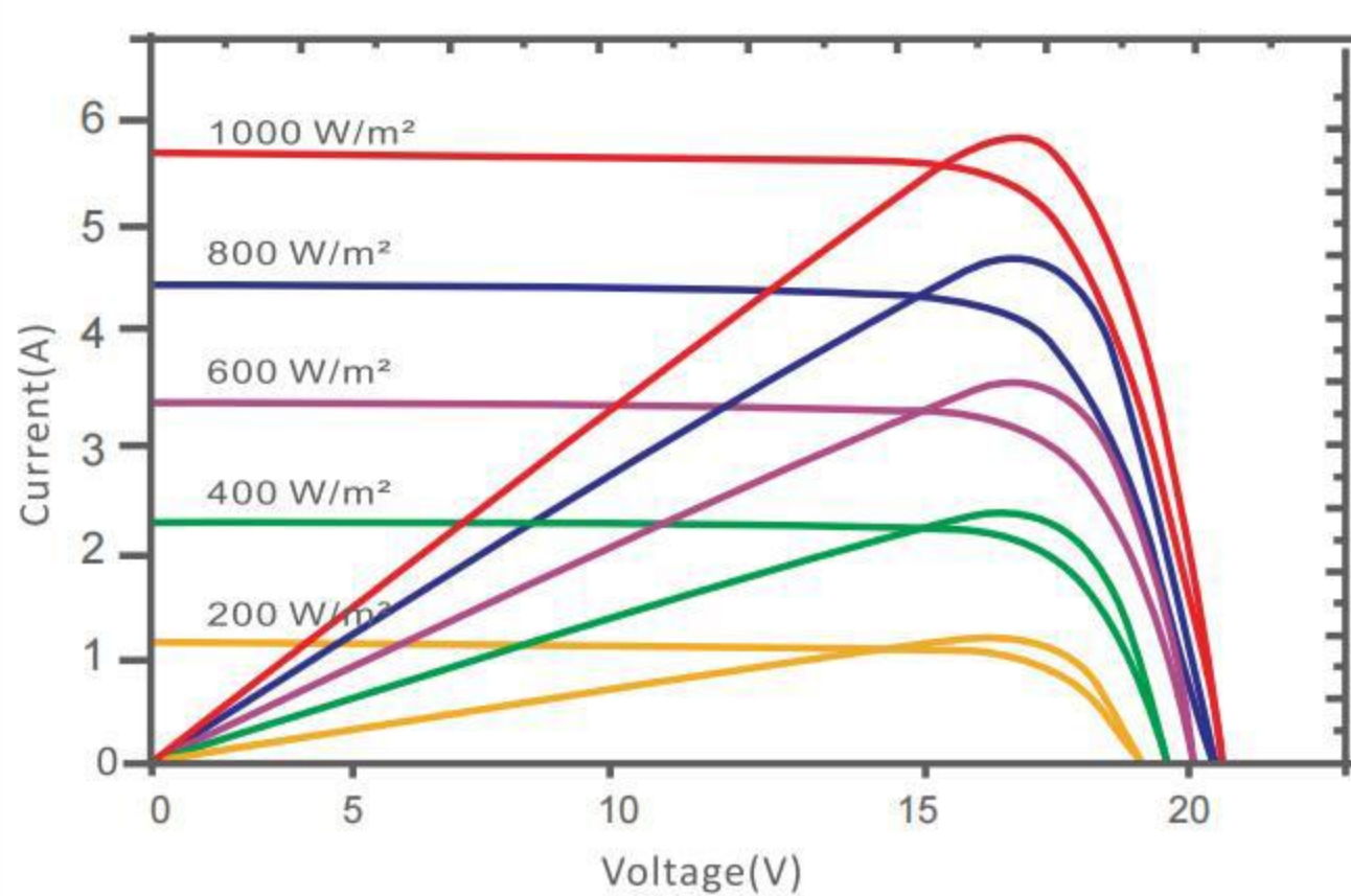
I-V characteristics at different irradiances
