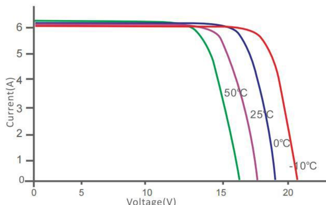
I-V characteristics at different temperature
